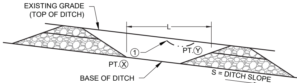
DETAIL FOR SPACING BETWEEN CHECK DAMS
