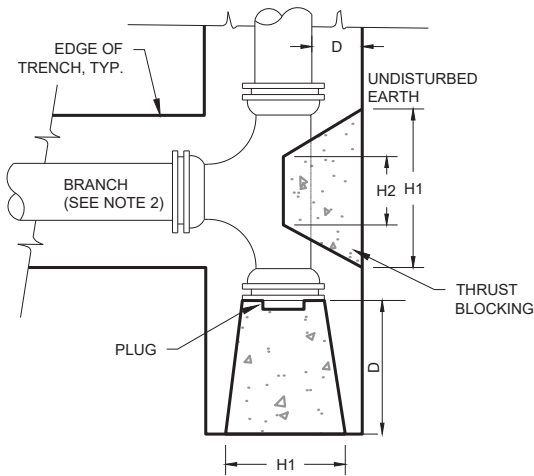
TEES, CROSSES AND PLUGS
