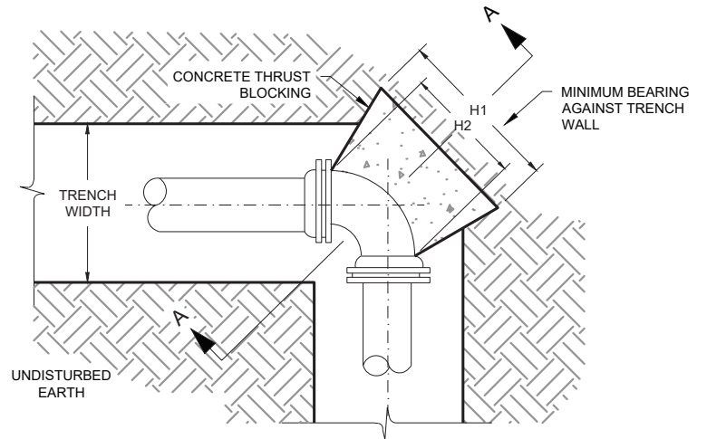
HORIZONTAL BENDS
