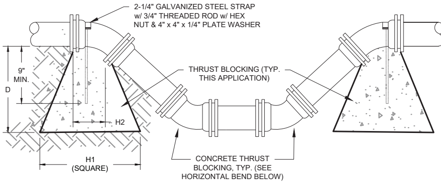
VERTICAL BENDS
